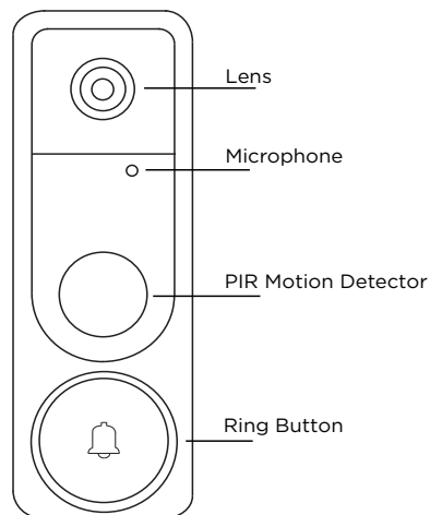
Figure 2: Video Doorbell Layout
